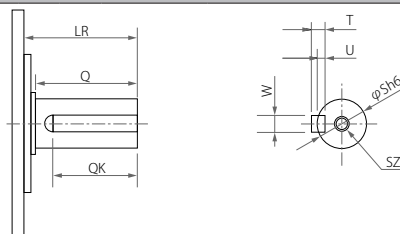
Shaft extension specifications [with key, tapped]
