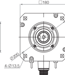
GYL motor (without brake)
