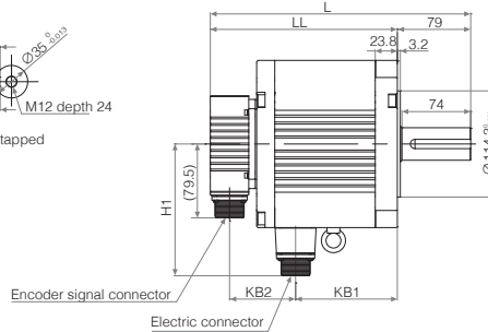
GYL motor (without brake)
