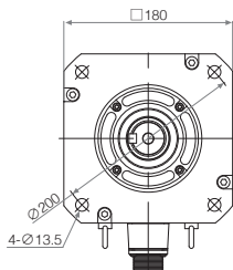
GYL motor (without brake)
