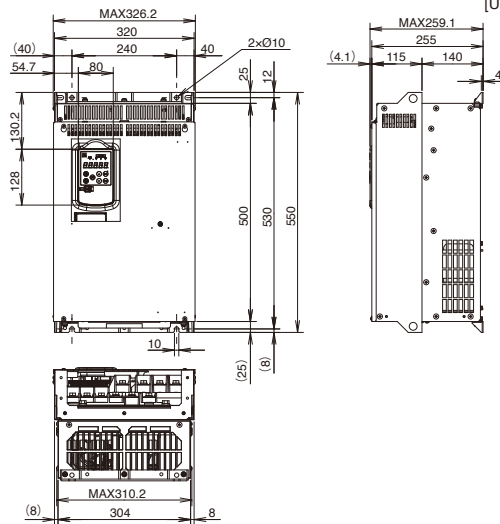
Type FRN30G2□-2J, FRN30G2□-4J, FRN37G2□-4J FRN37G2P-2J, FRN37G2P-4J~55G2P-4J
