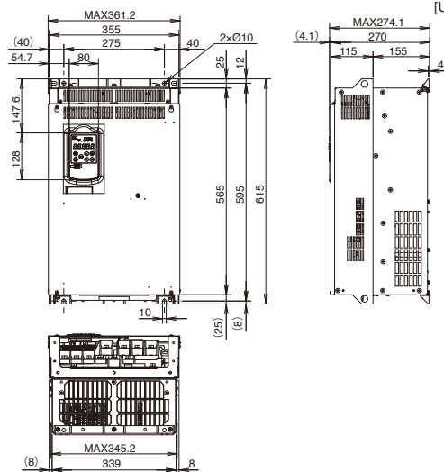
Type FRN37G2□-2J, FRN45G2□-4J FRN45G2P-2J~55G2P-2J, FRN75G2P-4J
