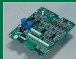
PMPG interface card (optional)
